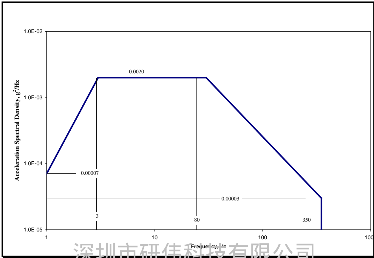
Figure 514.7C-11. Category 11 - Rail cargo vibration exposure.
