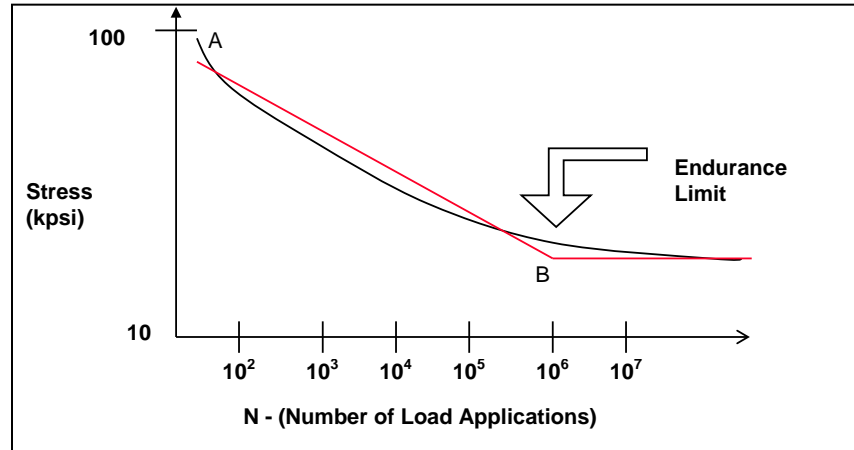
Figure 514.7F-2. S/N curve.
