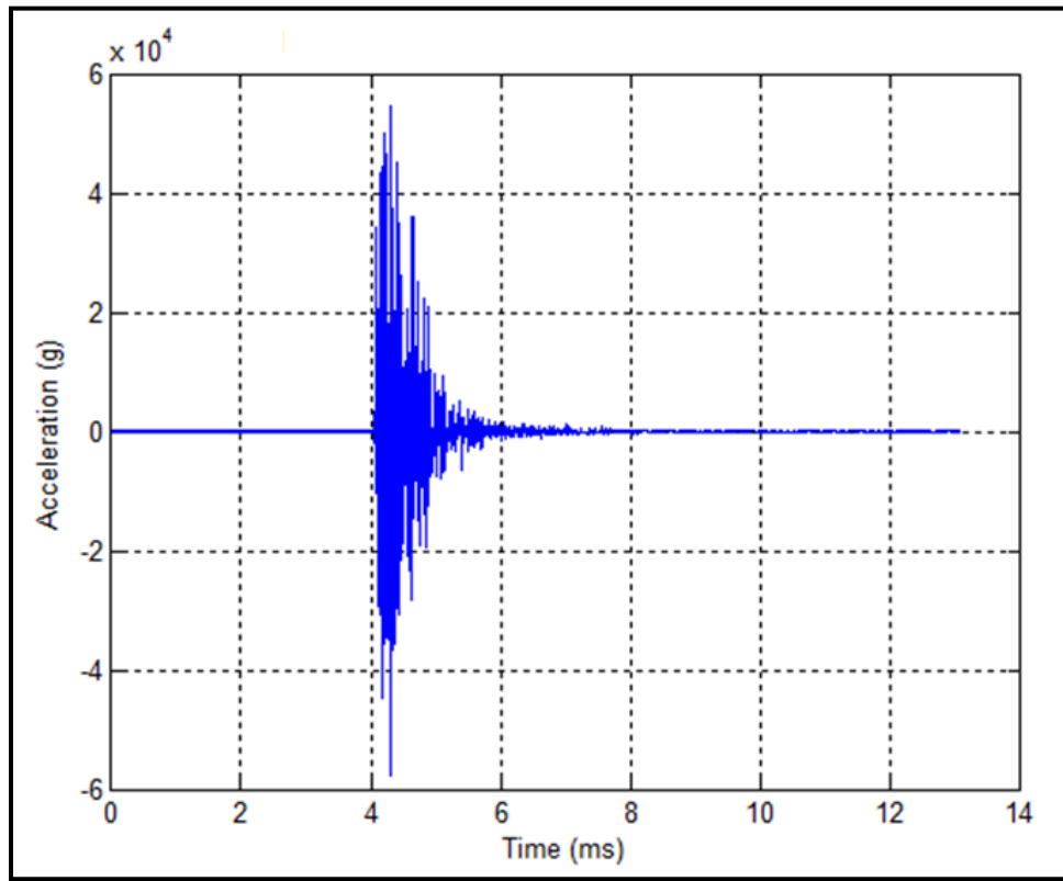
Figure 517.2A-14. A near-field gyroshock acceleration time history.
