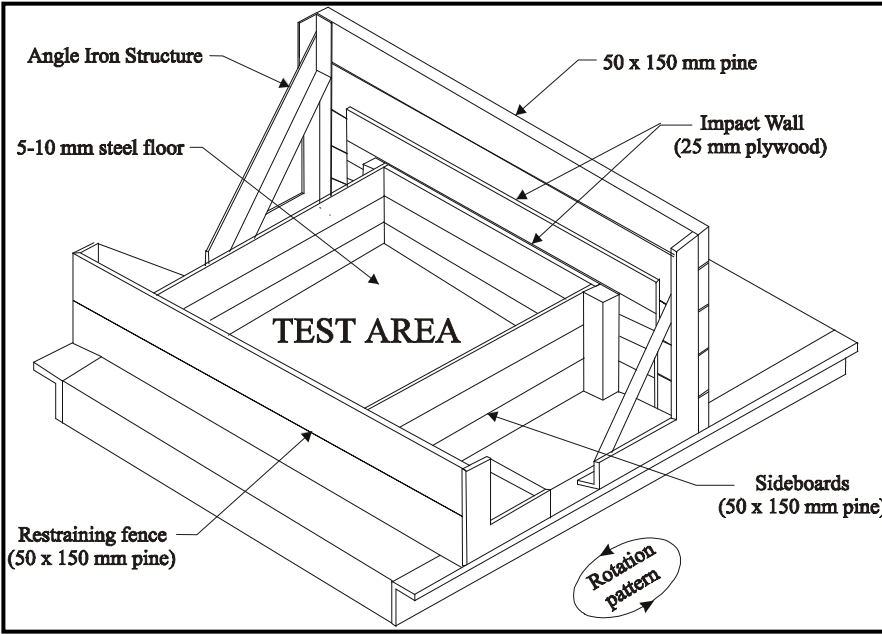
Figure 514.7C-5. Category 5 - Loose cargo test setup.
