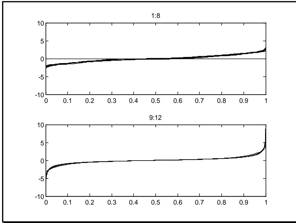
Figure 519.7B-14. Cumulative coefficient distribution for details Level 1:8 and 9:12.
