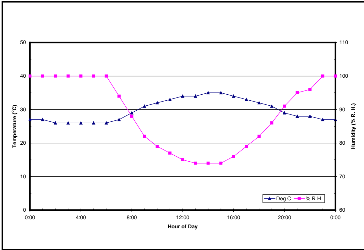
Figure 507.6-5. Natural Cycle B2 -- Cycle high humidity
