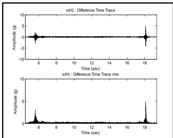
Figure 525.1A-9a. Difference Exciter (H).
