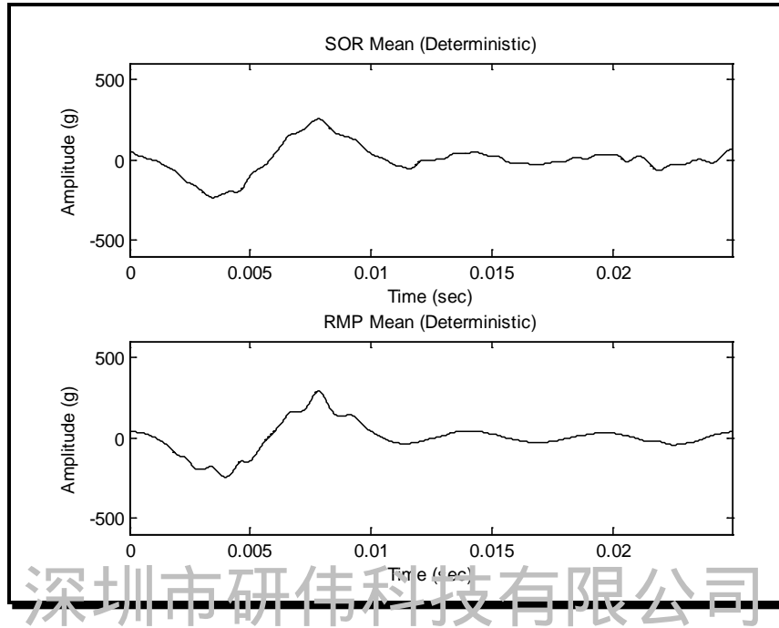
Figure 519.7C-9a. Pulse ensemble statistics - deterministic component m(t) .
