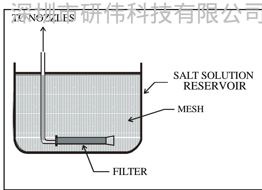
Figure 509.6-1. Location of salt solution filter.
