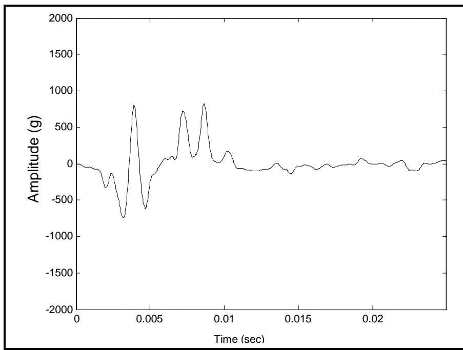
Figure 519.7C-5b. Sample model (single pulse) ( \text{RMP } x(t) = r(t)m(t) ).
