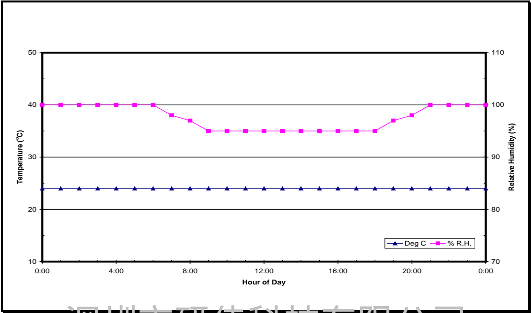
Figure 507.6-4. Natural Cycle R1 - Constant high humidity.
