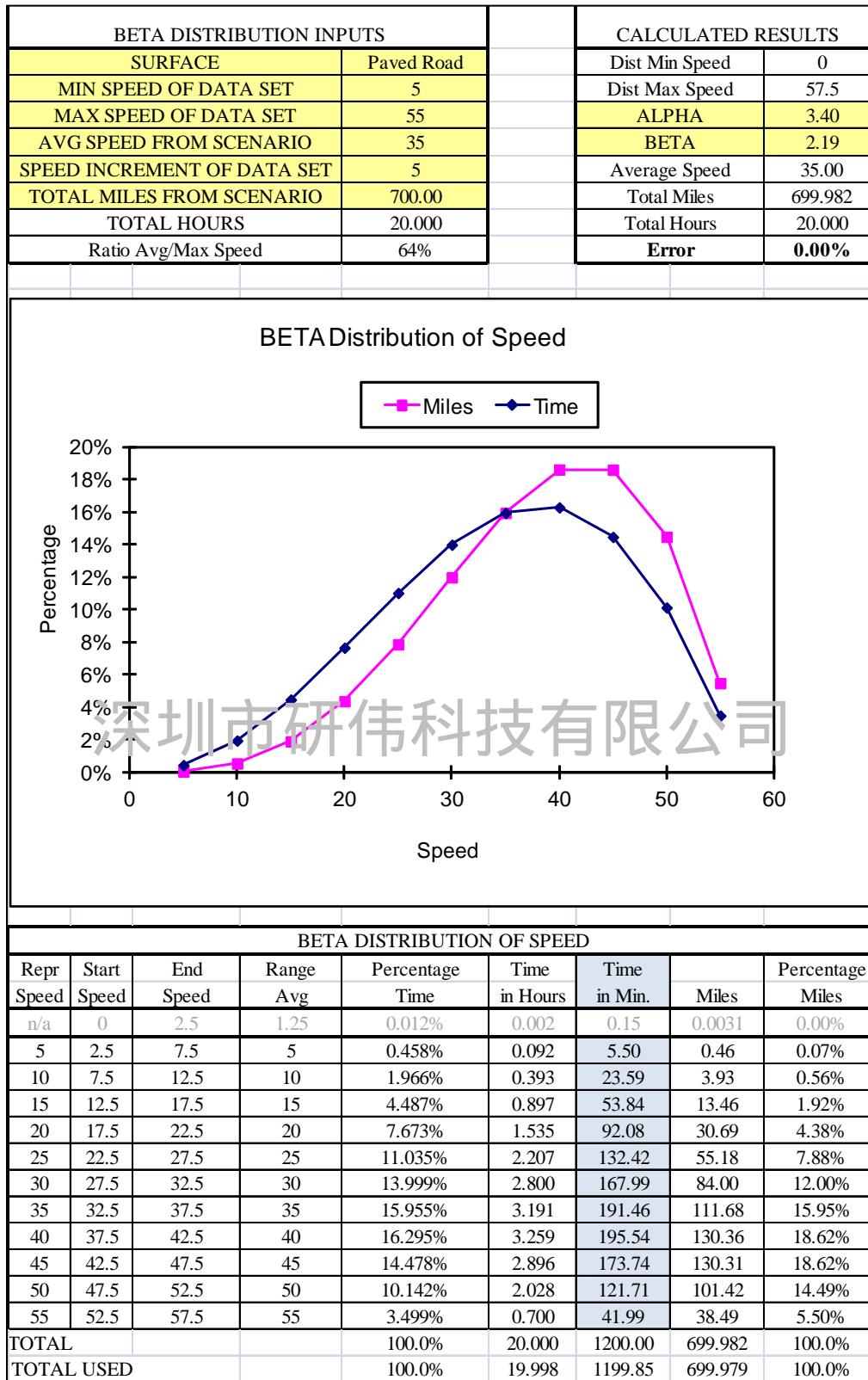
Figure 514.7F-1. Sample beta distribution (wheeled vehicle).
