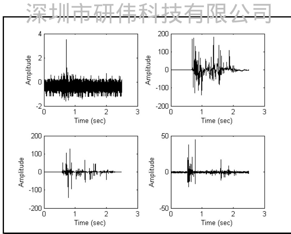
Figure 516.7A-7. Measurement input overdriving the signal conditioning with clipping.
